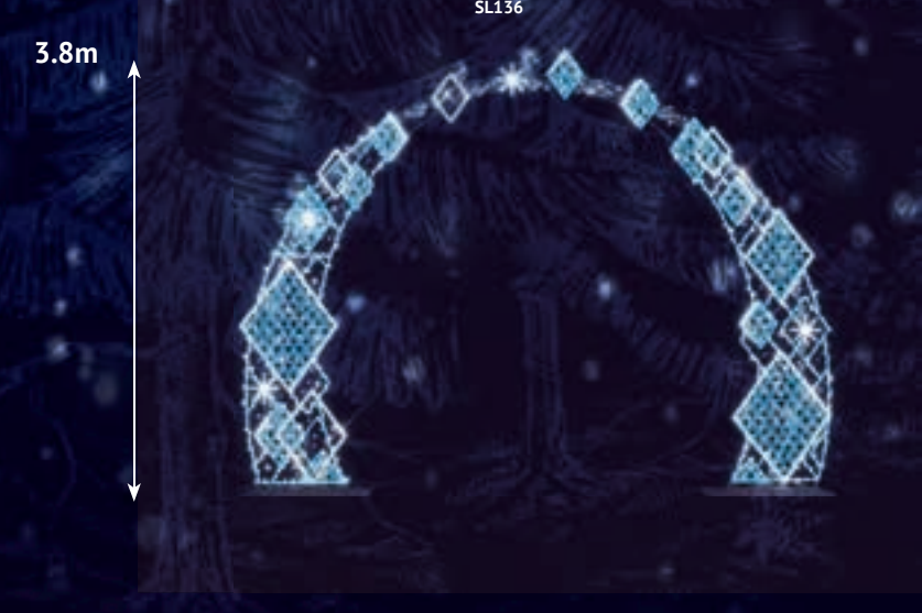
GX252L- TRADI ARC ◆ 4.6m ◆ 5.9m ▮ 1.0m 🏠 382kg ⚡ 568W 🔵 🔵 STARS&FLASH 25 TO ORDER SL136- QUADRILLE ARCH ◆ 3.8m ◆ 4.9m ▮ 1.0m 🏠 81.5kg ⚡ 60W 🔵 🔵 XLED & FL900E&FLASH 25 TO ORDER
